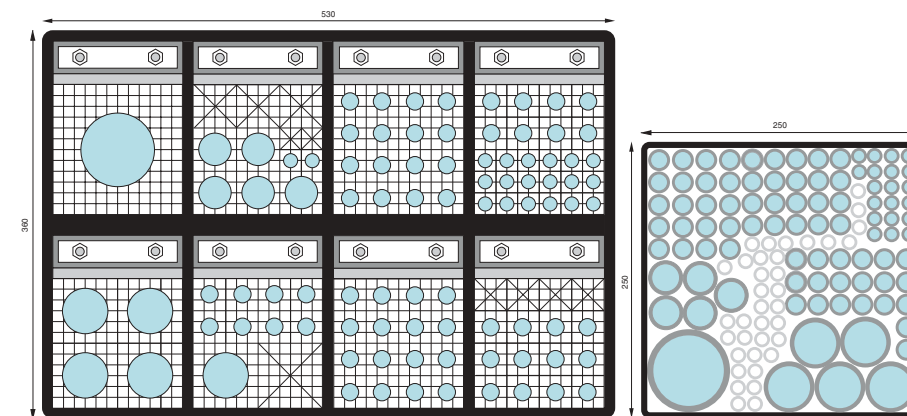
same amount of cables in less than half the conduit size with RISE®
